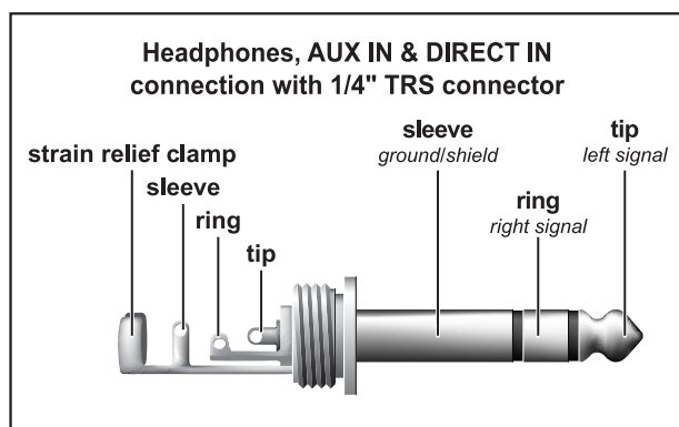
Fig. 4.4: 1/4" TRS connector for headphones operation
