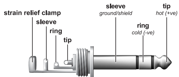
Fig. 4.3: 1/4" TRS connector
