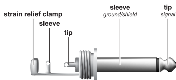
Fig. 4.2: 1/4" TS connector
