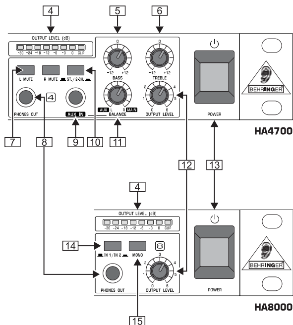
Fig. 2.2: Individual headphones amplifier sections
