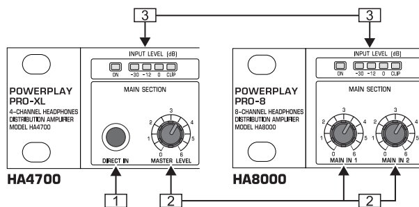
Fig. 2.1: Input section
