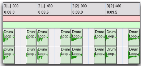
After quantizing
