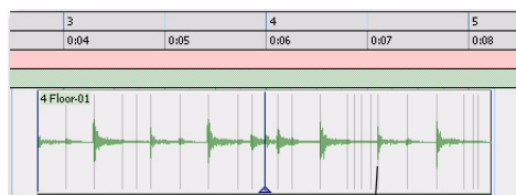
After warping
