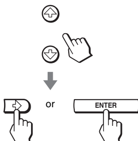
Pop-up menu
