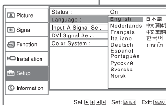
Setting menu
