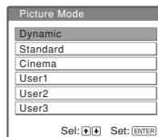
Adjustment menu
